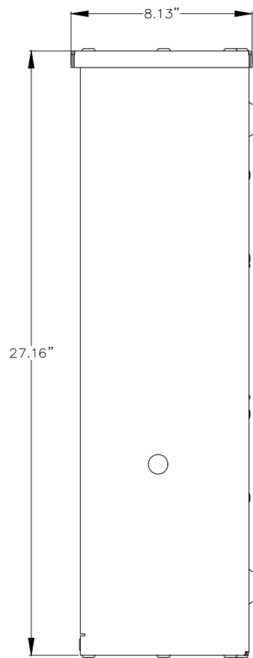
RHS VIEW
