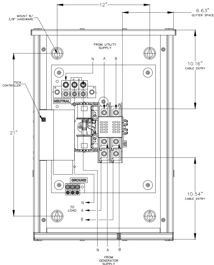
INTERIOR FRONT VIEW (DOOR NOT SHOWN)
