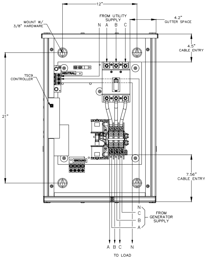
INTERIOR FRONT VIEW (DOOR NOT SHOWN)
