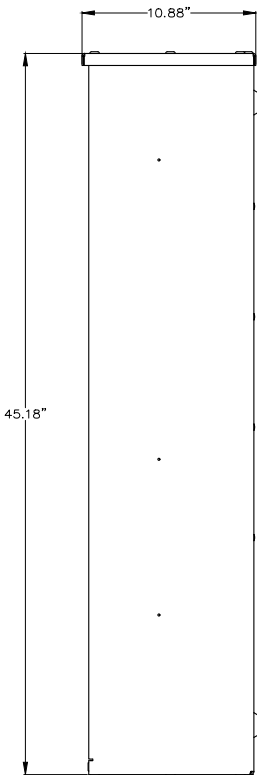
RHS VIEW
