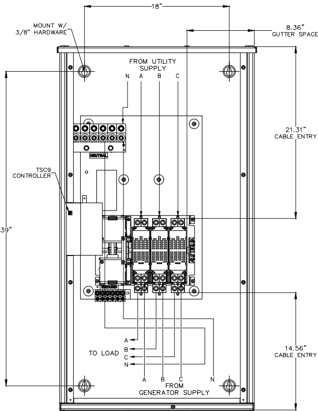
INTERIOR FRONT VIEW (DOOR REMOVED)
