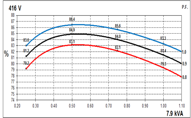
60Hz Curves
