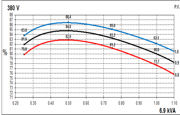
50Hz Curves
